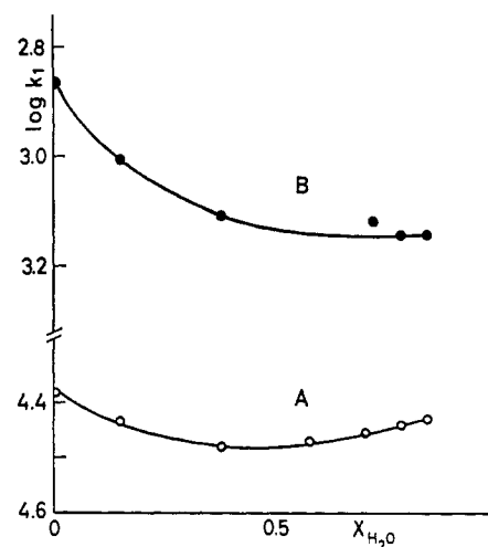
Figure 2. Plots of log k 1 vs. X H 2 O : (A) for 3-Br; (B) for 3-OTs.
