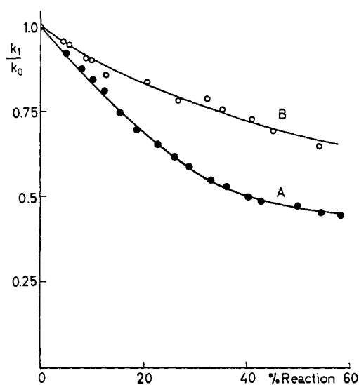
Figure 3. Plots of the relative decrease of k_1 of the first-order equation (expressed as k_1/k_1^0 ) with the progress of the reaction of 3-Br. The points are experimental and the lines were calculated from eq 8: (A) 0.0105 mol l. -1 of 3-Br in 100% TFE at 45° with \alpha = 290 ; (B) 0.0157 mol l. -1 of 3-Br in 90% TFE at 35° with \alpha = 110 .
